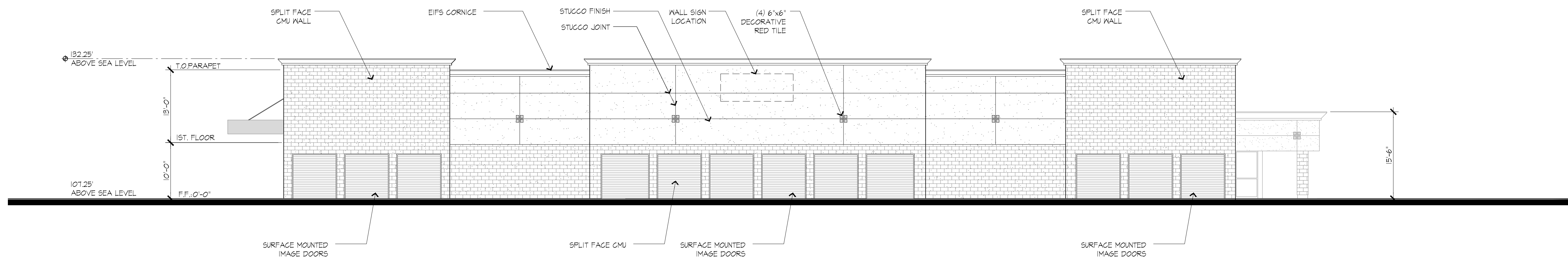
EAST ELEVATION
